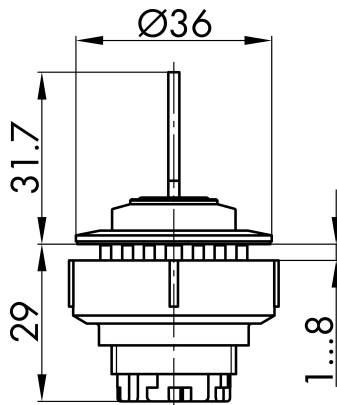
→ Dimensional drawing
