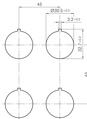
→ Cutout dimensions
