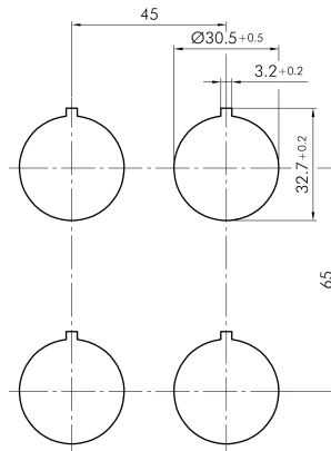
→ Cutout dimensions
