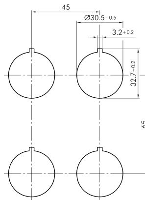
→ Cutout dimensions
