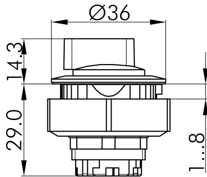
→ Dimensional drawing
