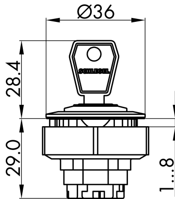
→ Dimensional drawing
