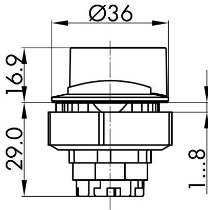
→ Dimensional drawing
