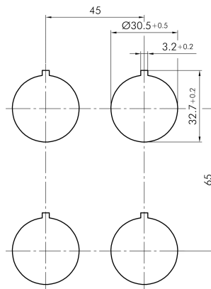
→ Cutout dimensions
