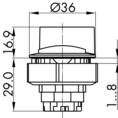
→ Dimensional drawing
