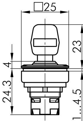
→ Dimensional drawing
