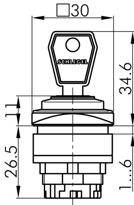
→ Dimensional drawing
