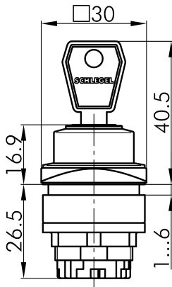
→ Dimensional drawing
