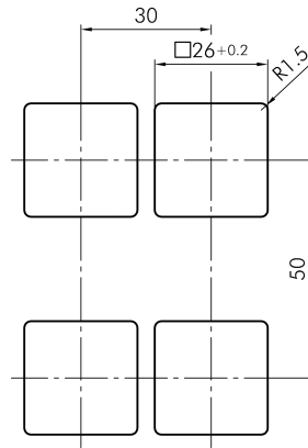
→ Cutout dimensions
