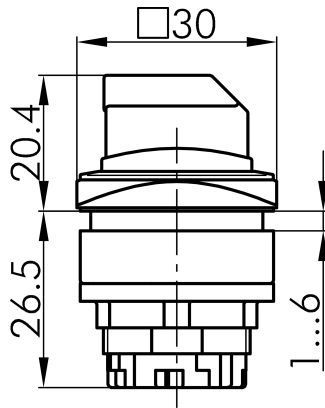
→ Dimensional drawing
