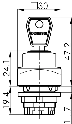
→ Dimensional drawing
