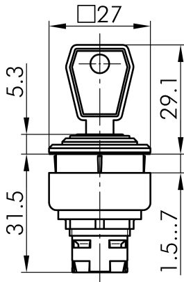
→ Dimensional drawing
