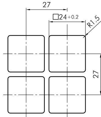
→ Cutout dimensions
