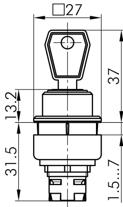
→ Dimensional drawing
