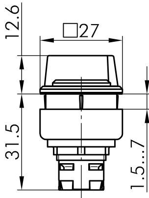
→ Dimensional drawing
