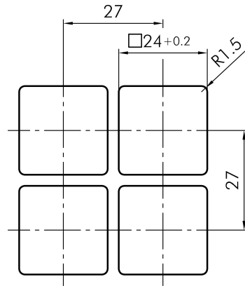
→ Cutout dimensions
