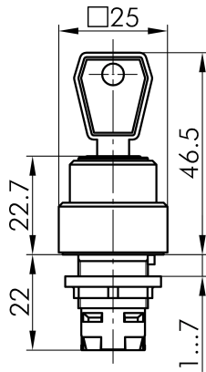
→ Dimensional drawing
