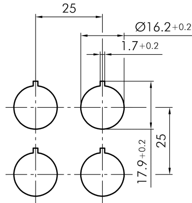
→ Cutout dimensions
