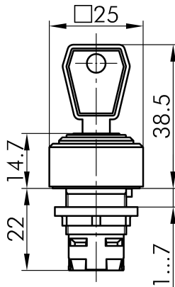
→ Dimensional drawing
