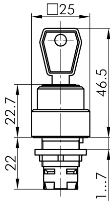
→ Dimensional drawing
