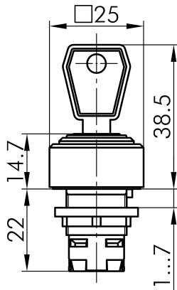
→ Dimensional drawing
