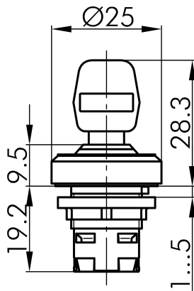
→ Dimensional drawing
