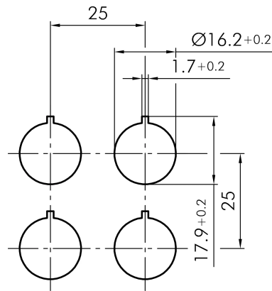
→ Cutout dimensions
