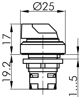
→ Dimensional drawing
