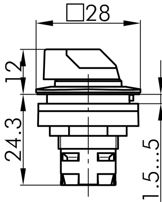
→ Dimensional drawing
