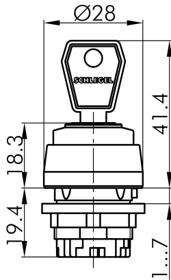
→ Dimensional drawing
