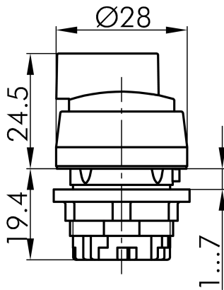
→ Dimensional drawing
