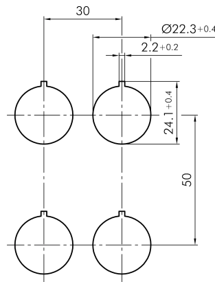
→ Cutout dimensions
