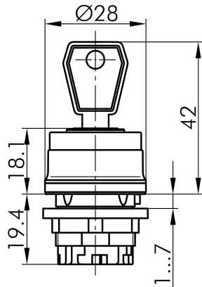
→ Dimensional drawing
