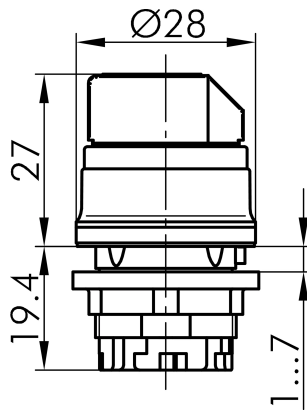
→ Dimensional drawing
