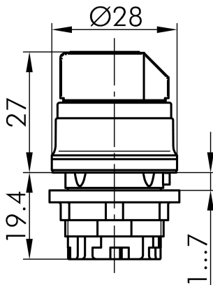
→ Dimensional drawing
