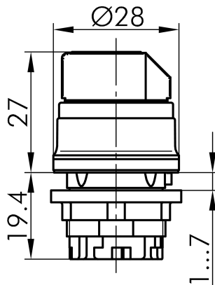
→ Dimensional drawing
