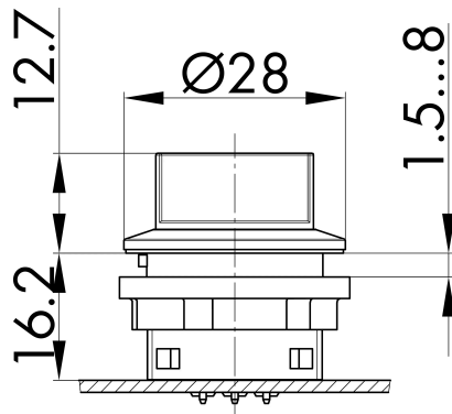
→ Dimensional drawing
